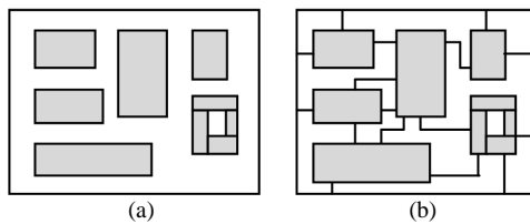
Fig. 6: Two sample descriptions (a): Layout of circuit blocks (b): Detailed routing
