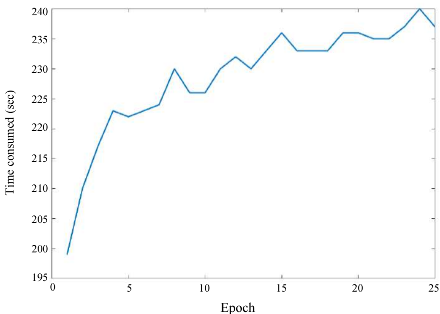
Fig. 9: Time consumed for training dataset in seconds
